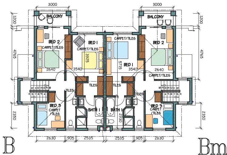
SECOND STOREY PLAN
